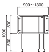
F-90 (10.1kg) FH-90 (9.9kg)
